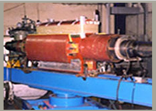
In- Situ Winding of Poles
