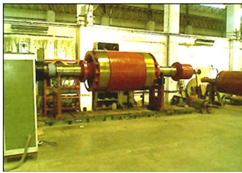
19.7 MVA Rotar Being Balanced
