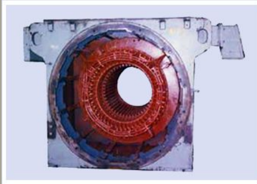
Rewinding of 2611 KW 11KV Stator Steel Industry
