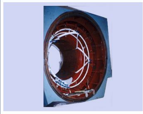
19.7 MVA Stator Being Rewound
